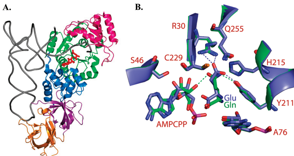
FIGURE 1: (A) Structure of E. coli GlnRS bound in a quaternary complex with tRNA Gln , glutamine, and the ATP analogue AMPCPP (12). The phosphates of AMPCPP are disordered in this structure. The Rossmann fold catalytic domain is colored green, the inserted domain that binds the tRNA acceptor end is bright pink, a helical subdomain following the Rossmann fold in primary sequence is shown in dark blue, and the proximal and distal anticodon binding domains are depicted in magenta and orange, respectively. (B) Superposition of the GlnRS active site in quaternary complexes bound to tRNA Gln , AMPCPP and either cognate glutamine (green) or noncognate glutamate (blue). Selected hydrogen bonds are shown as dotted lines. Both bound glutamine and glutamate participate in a hydrogen bond with Tyr211, but only cognate glutamine accepts a hydrogen bond from the 3'-OH group of ATP. Glutamate also makes direct electrostatic hydrogen bonds with Arg30.
