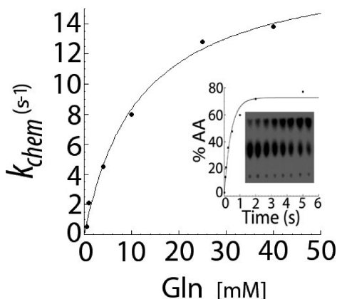
FIGURE 4: k_{\text{obs}} dependence on the glutamine concentration for the E257A GlnRS mutant, fit to a hyperbolic binding equation to determine the k_{\text{obs(max)}} and K_d values. The kinetic constant k_{\text{obs}} is very close to the wild-type GlnRS value, but the K_d (Gln) is elevated by 8.4-fold (see Table 2). The inset shows a TLC plate demonstrating the separation of substrate (AMP; center of TLC plate) and product (aa-AMP; top of TLC plate). The time points depicted are 0.02, 0.08, 0.12, 0.25, 0.5, 1.0, 2.0, and 5.0 s. The reactions were spotted at the bottom of the plate.
