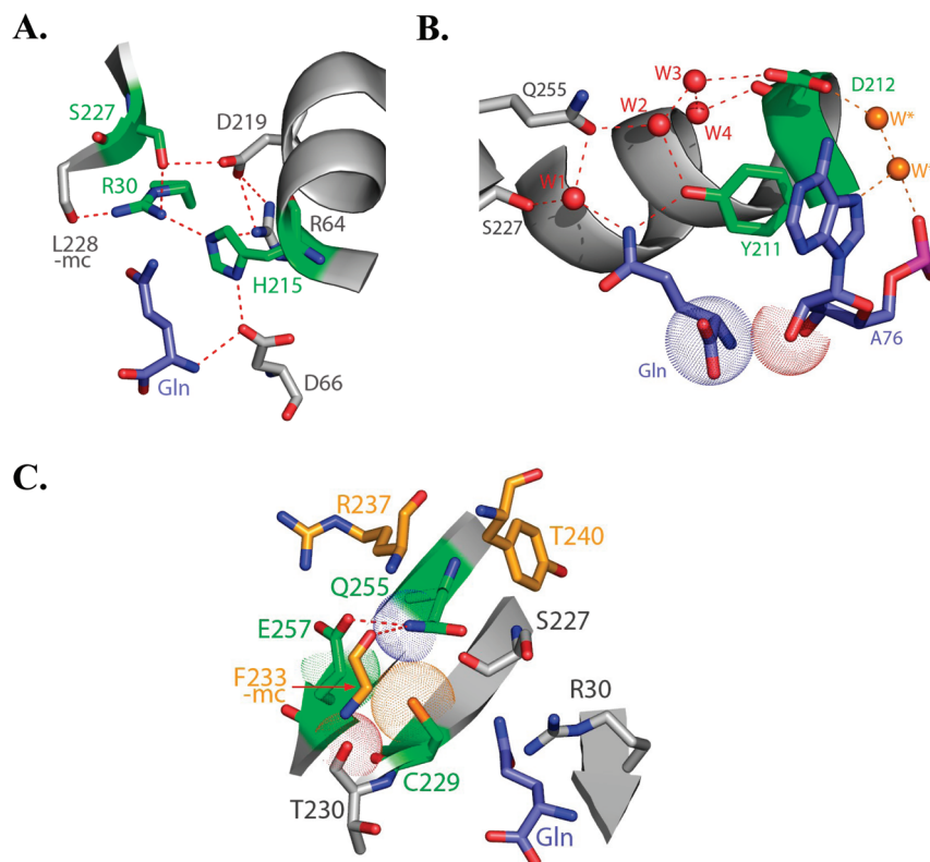
FIGURE 5: (A) Depiction of a portion of the glutamine binding pocket involving the interactions of Arg30, His215 and Ser227. Substrate glutamine is at the bottom, and hydrogen bonds are depicted in red dashed lines. The tautomer of His215 appears well-determined by interactions with the charged Arg30 and Asp66 groups. (B) Depiction of a portion of the glutamine binding pocket showing interactions of Tyr211 and Asp212. Waters labeled as W*, in yellow, are outside the immediate glutamine binding pocket and bridge Asp212 with the 3'-A76 nucleotide of tRNA. Juxtaposition of the substrate glutamine (bottom) with tRNA-A76 is depicted with van der Waals surfaces (bottom). (C) Depiction of a portion of the glutamine binding pocket showing interactions of Glu255, Cys229 and Glu257. Again, substrate glutamine is at the bottom of the drawing and selected hydrogen bonds are depicted as red dashed lines.
